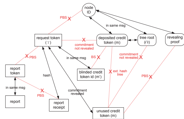
Fig. 7. The linkability between different components. Rounded rectangles (rectangles) denote the items transmitted with the node's real identity (random pseudonyms). The texts along solid arrows (dashed lines) explain the reason why the two connected items are linkable (unlinkable).
